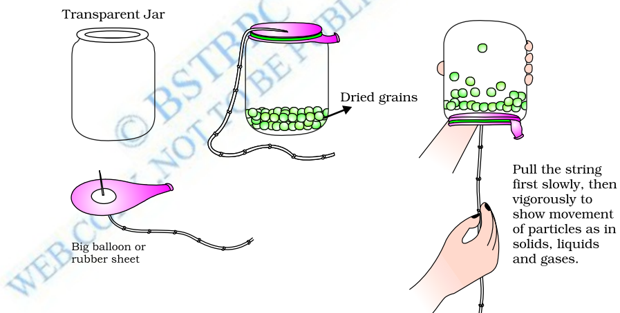
Fig. 1.10: A model for happy converting of solid to liquid and liquid to gas.
